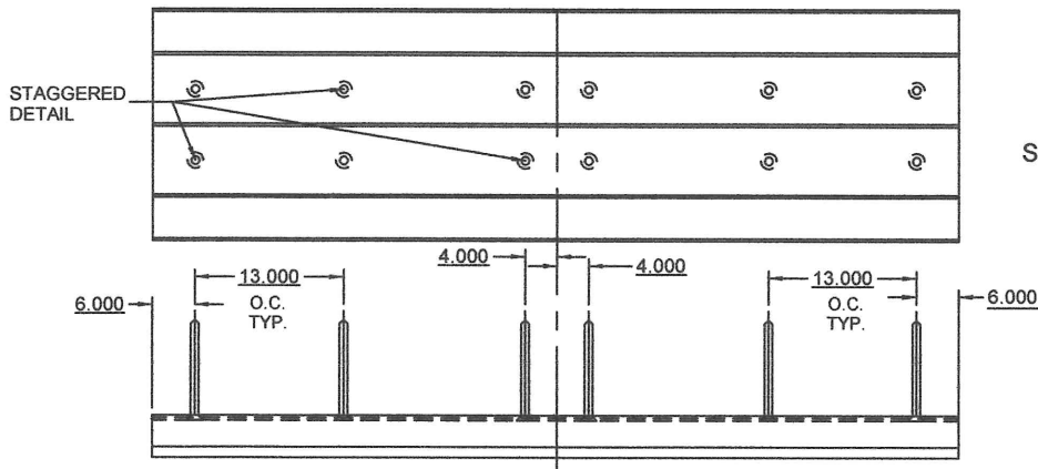
TYPICAL ANCHOR DETAIL AT INTERLOCK OR ASTRAGAL
